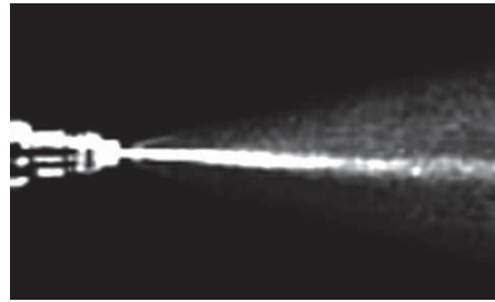
Injector spray pattern before P.i. treatment.
